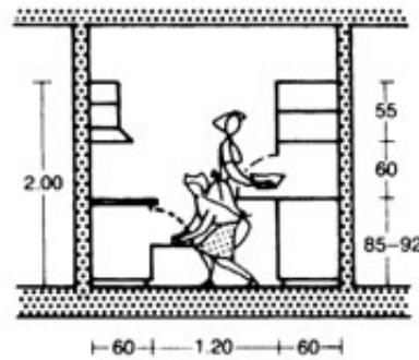
⑦ Side-by-side working
