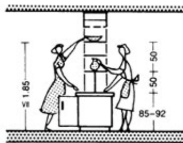
⑥ Hatch between kitchen and dining room
