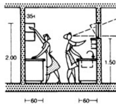
④ Worktops and storage 60 cm deep
